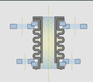
PTFE NORMAL BELLOW (GLASS/METAL) SLEEVE
