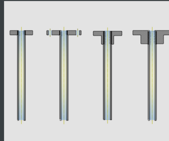
PTFE DROP WITH THREADED BUSH
