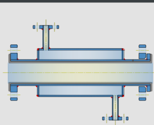
HALF JACKETED PIPE WITH FLANGE NOZZLE
