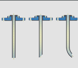
PTFE DROP TUBE, SINGLE PIECE WITH FLANGE
