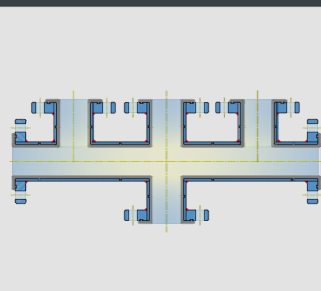
HEADER / MANIFOLD
