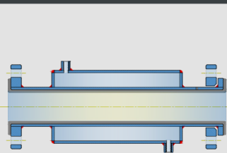
HALF JACKETED PIPE WITH NIPPLE NOZZLE
