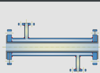
FULL JACKETED PIPE WITH FLANGE NOZZLE
